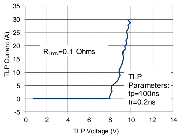
Figure 6: TLP Curve
